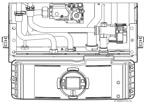
Fig. 4 Service position
