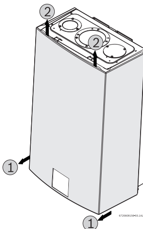
Fig. 2 Remove the front cover
