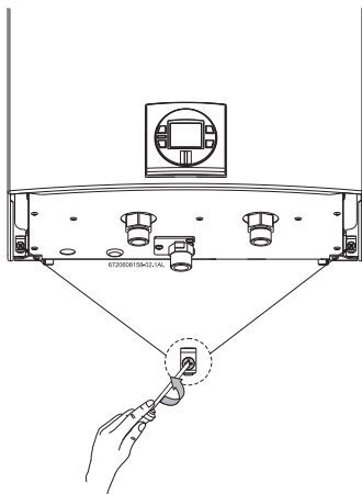
Fig. 1 Loosen the two screws
